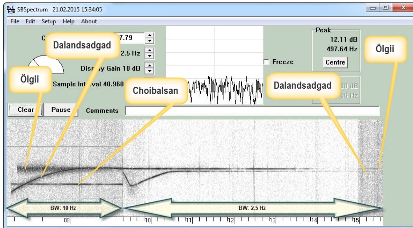
Figure 14: Here you see a sonagram from a recording of 209 kHz, concentrated on the two stations in close vicinity. The sonagram starts at a bandwidth of 10 Hz, showing also Choibalsan. After switching to a window of only 2,5 width, this transmitter falls out of it, because this station is 1,8 Hz down from this center frequency. You see two signals starting roughly at the same time (actually around 21:58 UTC). One has nearly no frequency drift over many hours, the other shows some drift at the start. This station also is slightly lower (-0,05 Hz) than the first station. This “lower” station fades out earlier. Hence, the station starting at a lower frequency should be Dalandsadgad with earlier local sunrise, the “higher” one Ölgii with later local sunrise and their new (May, 2012) transmitter TRAM150L of Transradio, Berlin.
