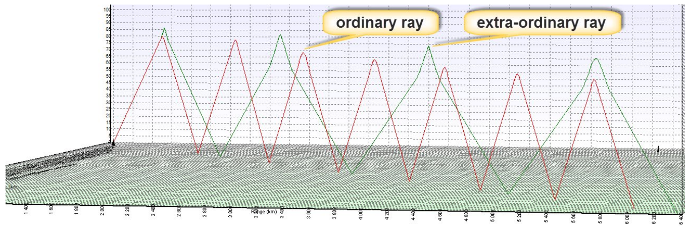
Figure 5: The path between Dalandsandgad and DK8OK on 209 kHz at 22:00 UTC. Only 3D-modeling shows the propagating extra-ordinary path with four hops. The ordinary path with its seven hops doesn't seem to contribute to propagation.
